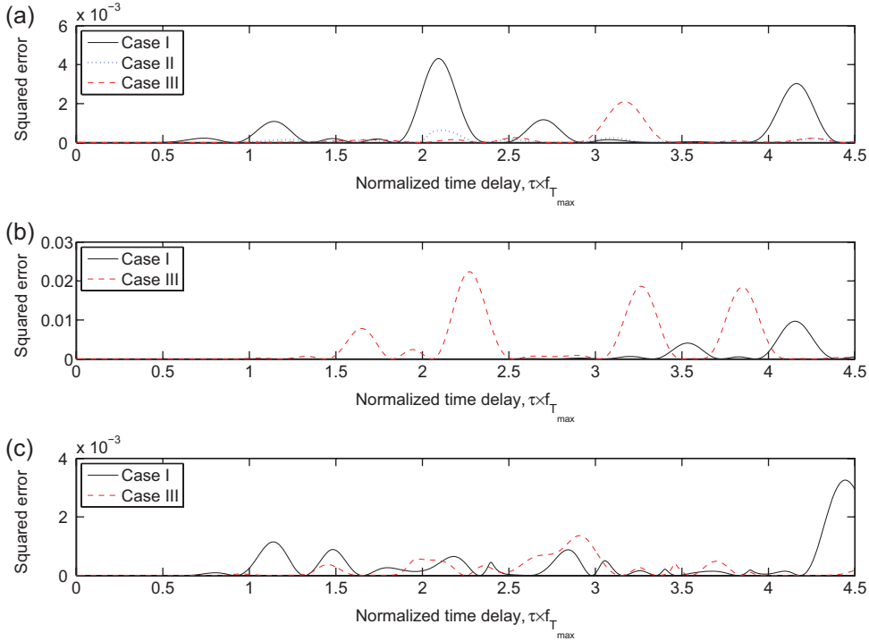
Fig. 3. Squared error in the CF of the proposed deterministic simulation model with k_T = k_R = 1 for different non-isotropic scattering M2M Rayleigh fading channels: (a) \mu_T = \mu_R = 110^\circ and \gamma_T = \gamma_R = 20^\circ ; (b) \mu_T = \mu_R = \gamma_T = \gamma_R = 0^\circ ; (c) \mu_T = 30^\circ , \mu_R = 160^\circ , \gamma_T = 10^\circ , and \gamma_R = 20^\circ .
