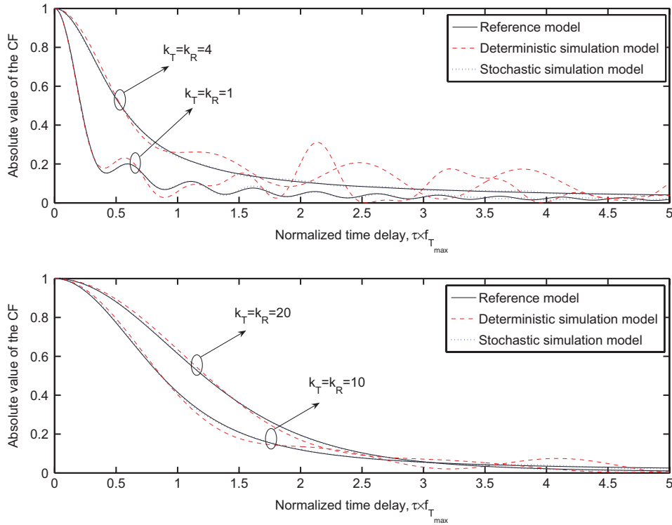
Fig. 6. Comparison between the CF of the reference model and the one of the proposed simulation models with \mu_T = \mu_R = 60^\circ and \gamma_T = \gamma_R = 30^\circ for various values of k_T and k_R .
