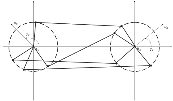
Fig. 1. Mobile-to-mobile scattering environment.
