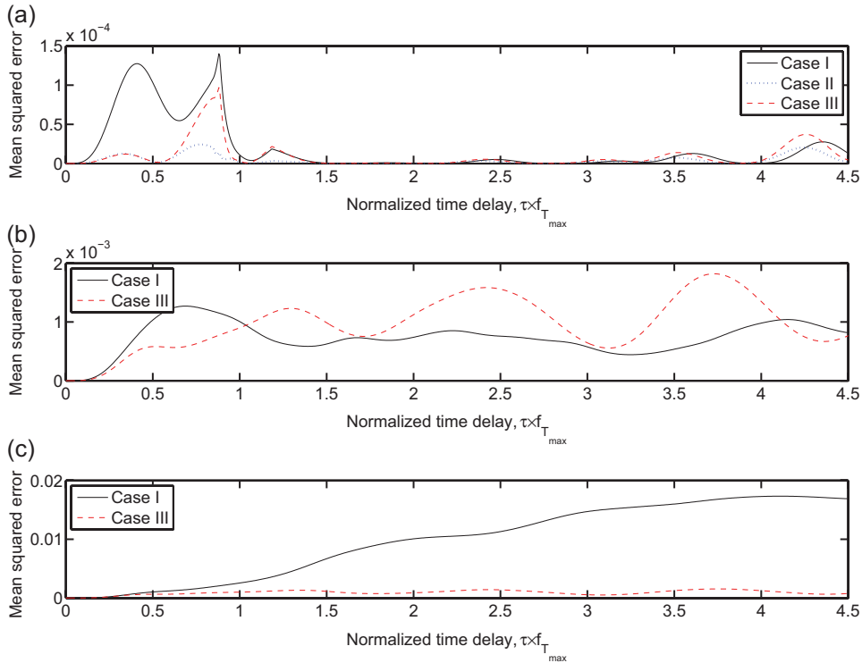
Fig. 4. Mean squared error in the CF of the proposed stochastic simulation model with k_T = k_R = 5 for different non-isotropic scattering M2M Rayleigh fading channels: (a) \mu_T = \mu_R = 110^\circ and \gamma_T = \gamma_R = 20^\circ ; (b) \mu_T = \mu_R = \gamma_T = \gamma_R = 0^\circ ; (c) \mu_T = 20^\circ , \mu_R = 10^\circ , \gamma_T = 10^\circ , and \gamma_R = 20^\circ .
