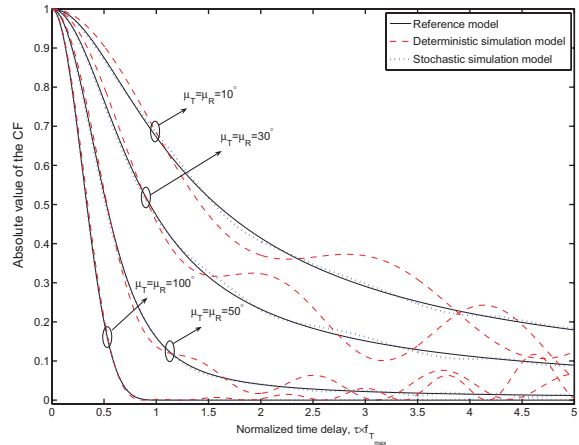
Fig. 5. Comparison between the CF of the reference model and the one of the proposed simulation models with k_T = k_R = 6 and \gamma_T = \gamma_R = 10^\circ for various values of the mean AoD \mu_T and mean AoA \mu_R .
