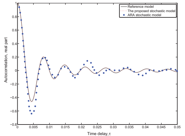
Fig. 2. Comparison between the proposed stochastic model and the ARA stochastic model proposed in Reference [22].
