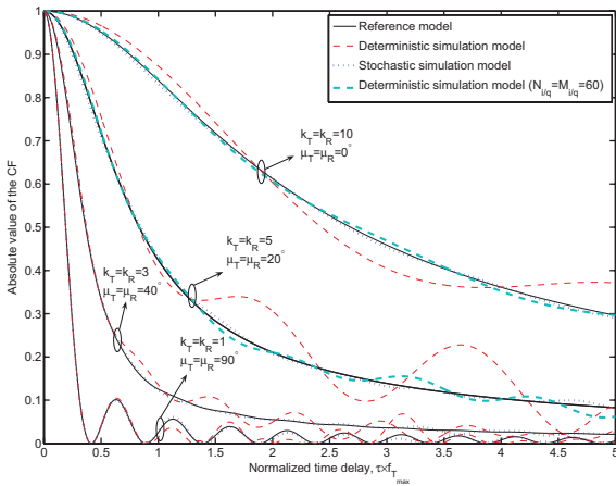
Fig. 7. Comparison between the CF of the reference model and the one of the proposed simulation models with \gamma_T = \gamma_R = 0^\circ for various values of k_T , k_R , the mean AoD \mu_T , and mean AoA \mu_R .
